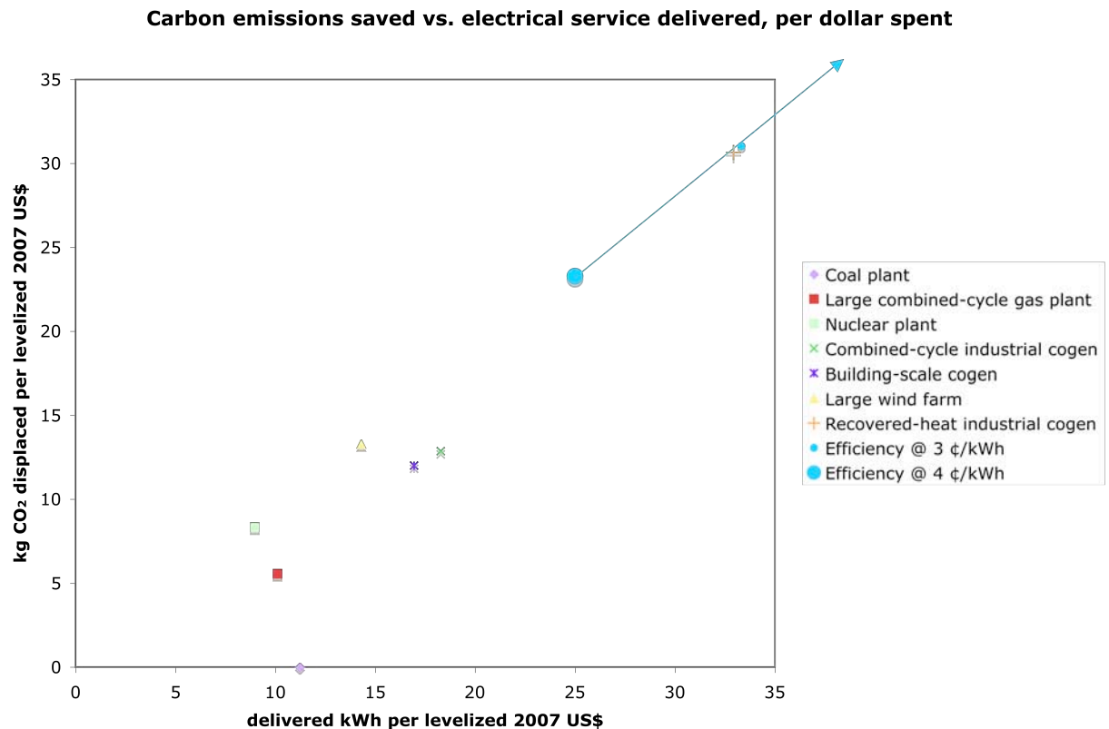
Fig. 5. The relative cost-effectiveness of different ways to spend a dollar to displace carbon emissions from coal-fired power plants (vertical axis) and to deliver new electrical services (horizontal axis). Options toward the lower left are worst for both priorities.
