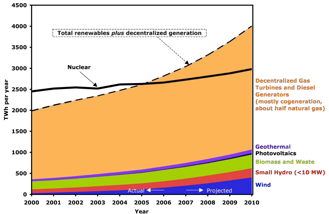
Low- or no-carbon worldwide electrical output (except large hydro)
